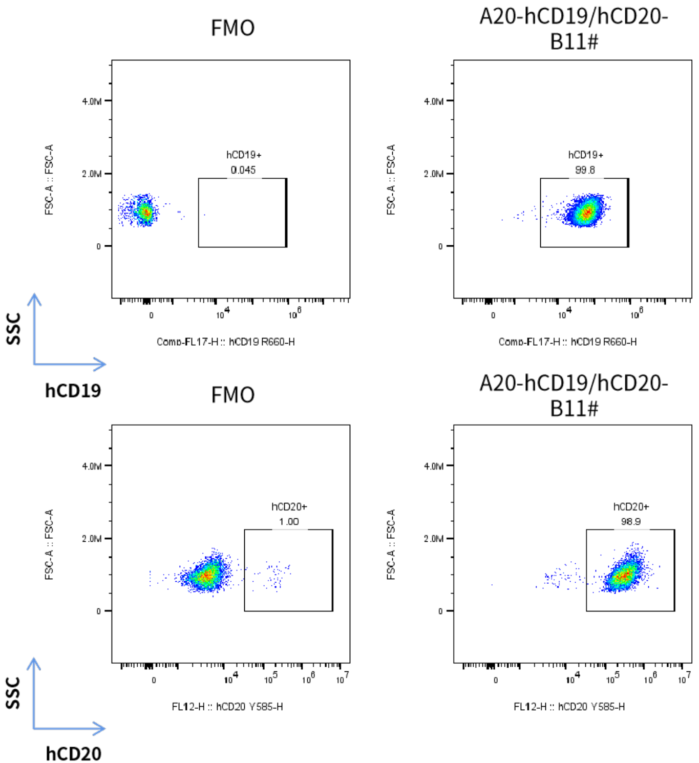
Fig1. hCD19/hCD20 expression on in vitro cultured cells of A20-hCD19/hCD20-Luc
