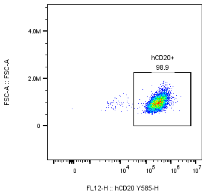
Fig2. hCD19/hCD20 expression on in vitro cultured cells of A20-hCD19/hCD20-Luc
